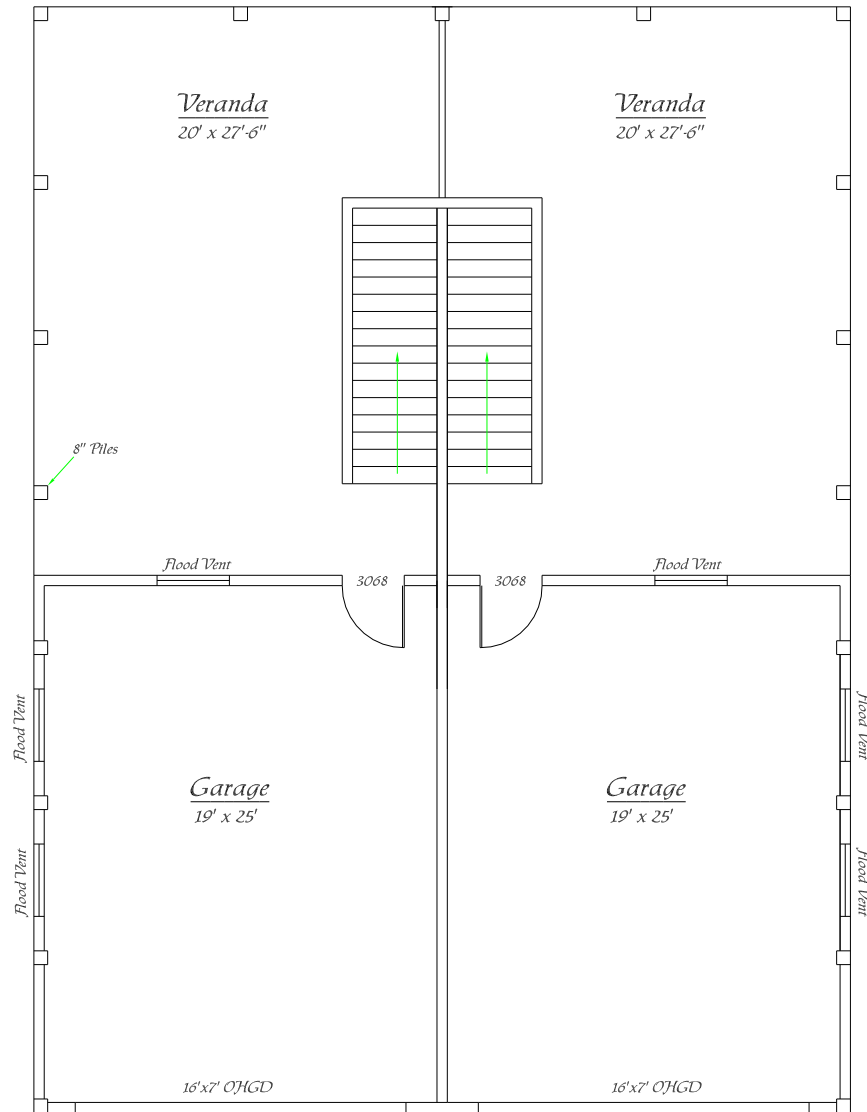
Ground Layout
